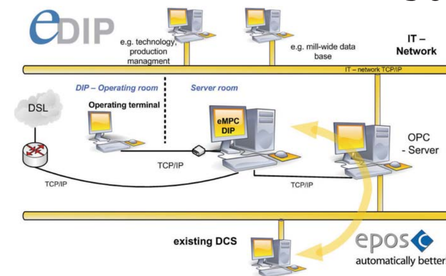
Technical integration of the eDIP-solution in the existing infrastructure
